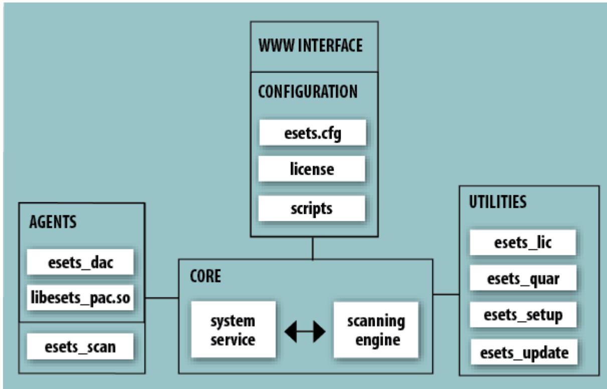
Figure 4-1. Structure of ESET File Security.
