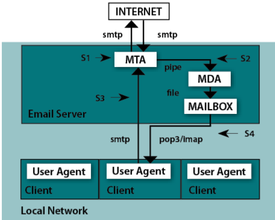
Figure 5-1. Scheme of UNIX OS email messaging system.
